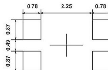
Recommended Land Pattern
